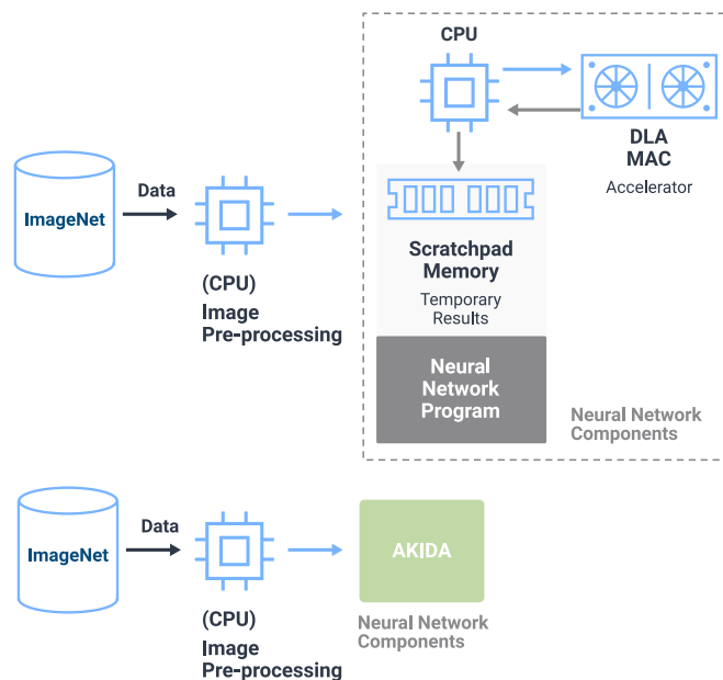
Figure 1: A traditional Neural Processing solution using a CPU, Deep Learning Accelerator, and external memory vs. the Akida solution as a fully integrated, purpose-built neural processor
