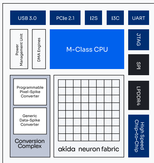
Akida AKD1000 SoC
