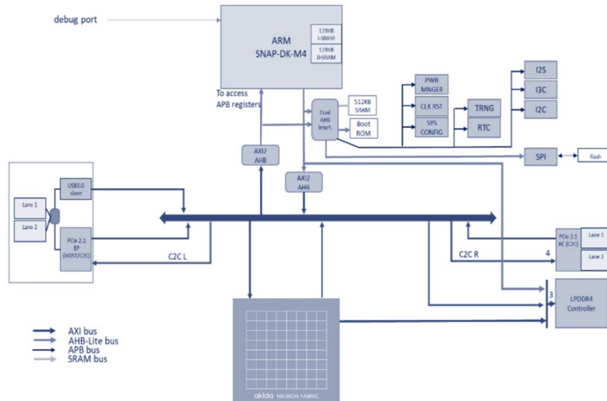
AKD1000 Block Diagram
